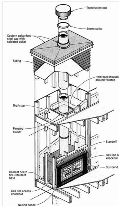
Illustration - 2 Prefabricated Chimney
